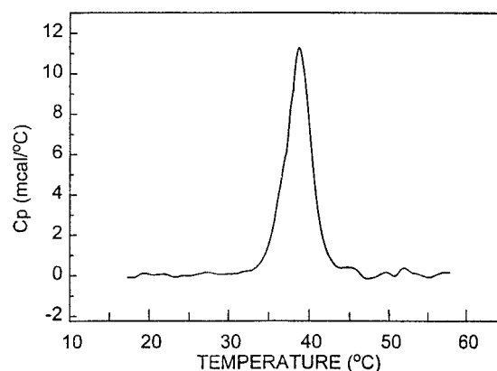
FIGURE 5 DSC thermogram of FFL. FFL was dissolved in 0.5 M glycylglycine buffer (pH 7.8) at 3 mg g -1 and scanned at 1.0°C min -1 .
