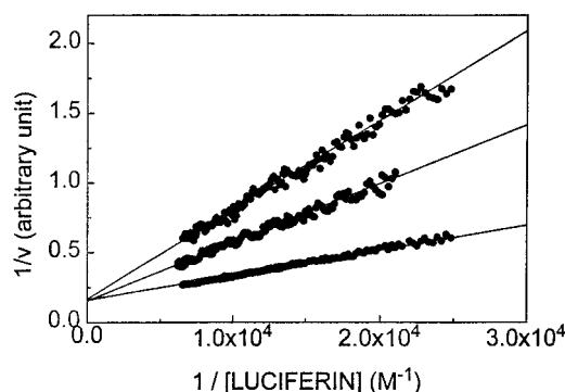
FIGURE 3 Lineweaver-Burk plots of myristic acid. Lineweaver-Burk plots were constructed by continuous infusion of luciferin under a steady-state condition by decelerating the reaction with the addition of pyrophosphate. The photomultiplier output was monitored by a Nicolet digital recording oscilloscope and downloaded onto floppy disks. The dilution effect (infusion volume) was corrected with a PC, and then the luciferin concentrations were converted into reciprocal form and extrapolated by linear regression with MicroCal Origin software. The lines are (from the bottom) control, 0.3 \mu\text{M} myristic acid, and 1.4 \mu\text{M} myristic acid. The K_i value was estimated by averaging three determinations. Myristic acid inhibited FFL in competition with luciferin with K_i = 0.53 \mu\text{M} .
